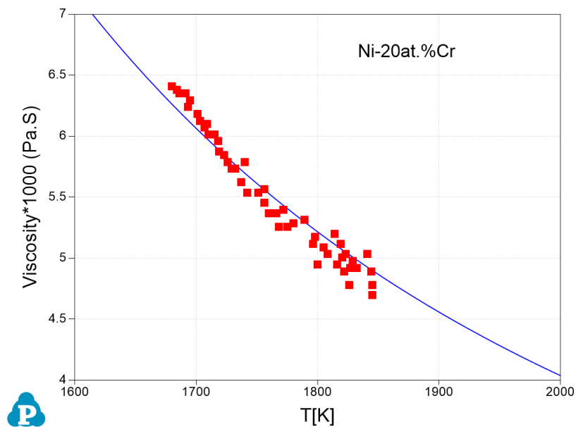
Figure 3.4: Viscosity of the Ni-Cr alloy
