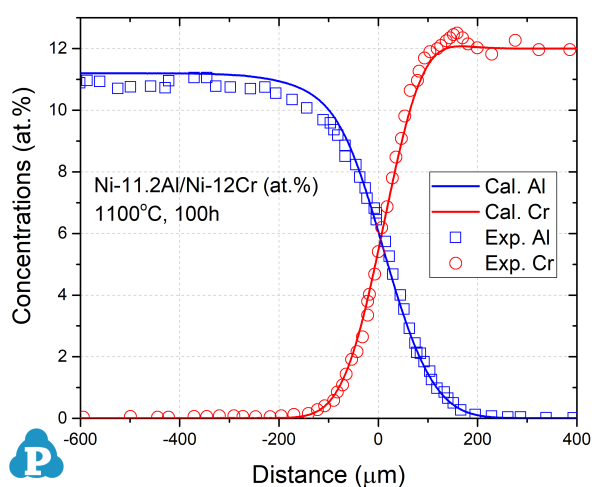
Figure 2.1: Concentration profiles of Ni-11.2Al/Ni-12Cr (at.%) at 1100 °C for 100h
