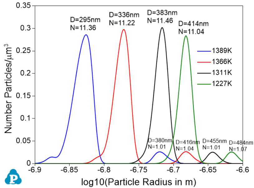
Figure 2.4: Simulated number densities of \gamma' particles when cooling to various temperatures with the cooling speed of 11K/m
