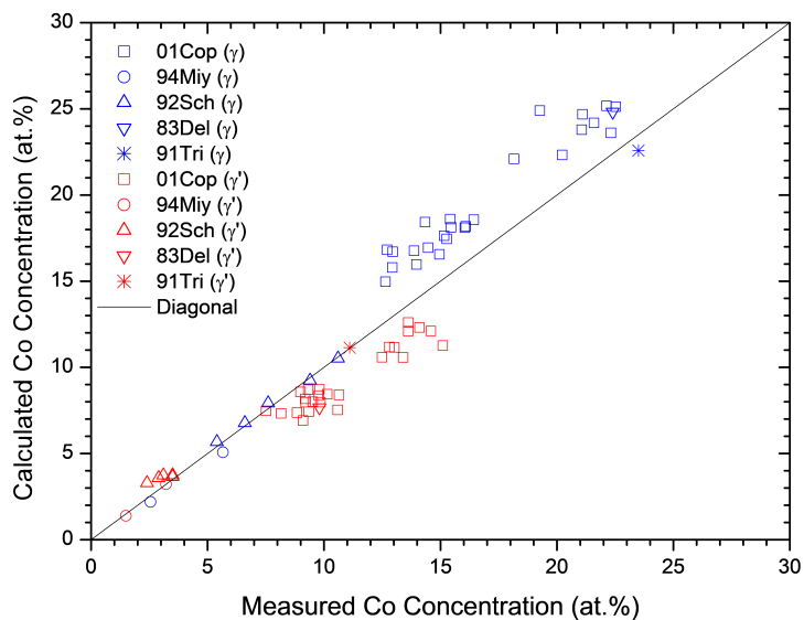
Figure 1.5: Comparison between the calculated and experimentally measured equilibrium compositions of Co in \gamma and \gamma' phases
