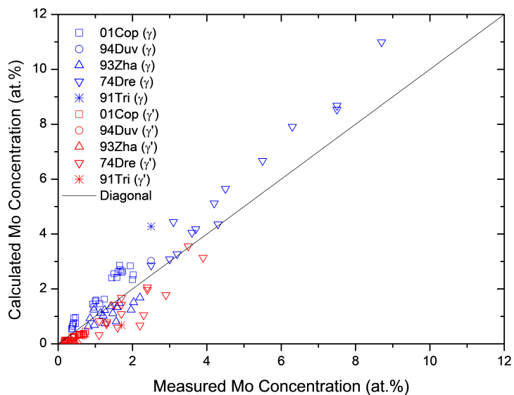
Figure 1.7: Comparison between the calculated and experimentally measured equilibrium compositions of Mo in \gamma and \gamma' phases
