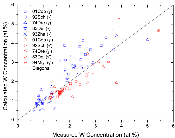
Figure 1.10: Comparison between the calculated and experimentally measured equilibrium compositions of W in \gamma and \gamma' phases
