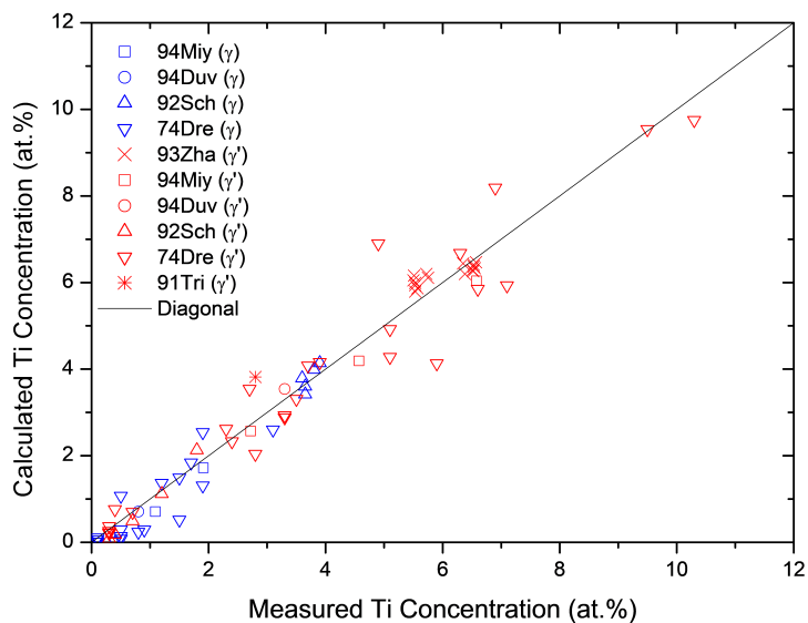
Figure 1.9: Comparison between the calculated and experimentally measured equilibrium compositions of Ti in \gamma and \gamma' phases
