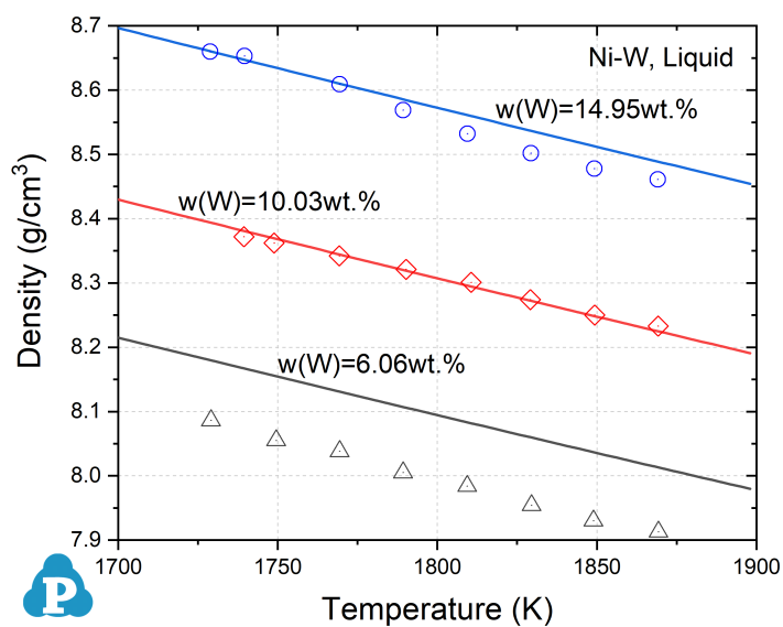
Figure 3.2: Density of Ni-W binary liquid mixture [2005Fan2]
