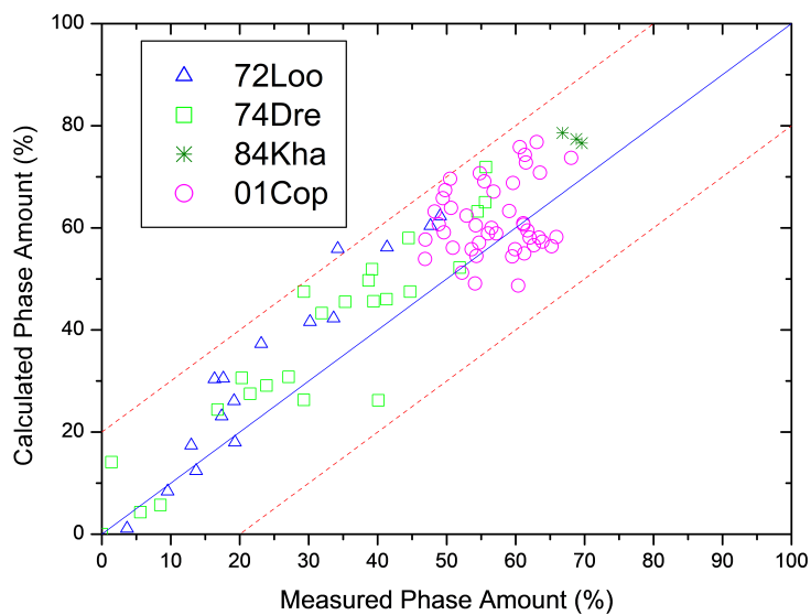
Figure 1.3: Comparison between the calculated and experimentally measured amounts of the \gamma' phase
