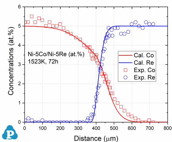
Figure 2.2: Concentration profiles of Ni-5Co/Ni-5Re (at.%) annealed at 1523K for 72h
