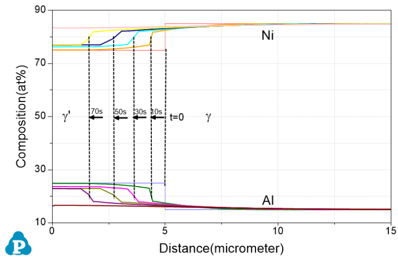
Figure 2.5: Simulated dissolution of \gamma' particle in Ni-Al binary system at 1200 °C
