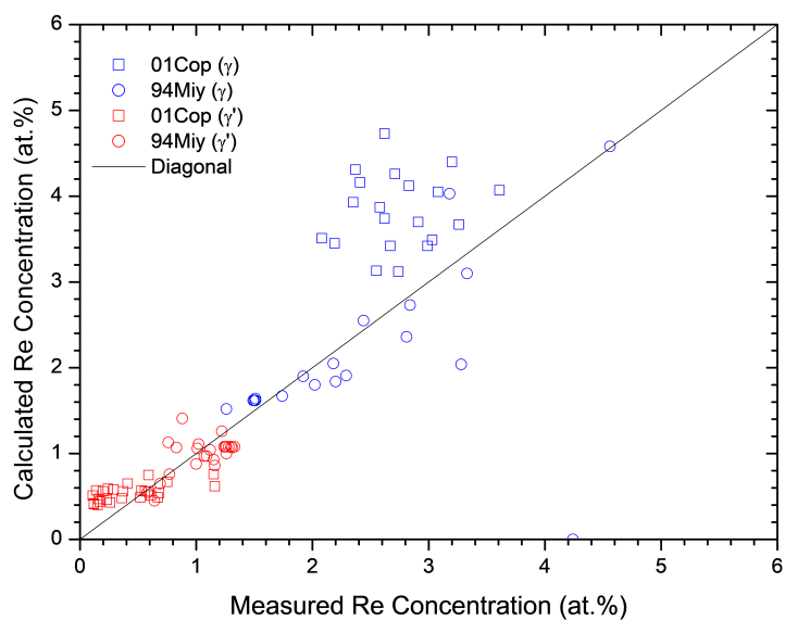
Figure 1.8: Comparison between the calculated and experimentally measured equilibrium compositions of Re in \gamma and \gamma' phases
