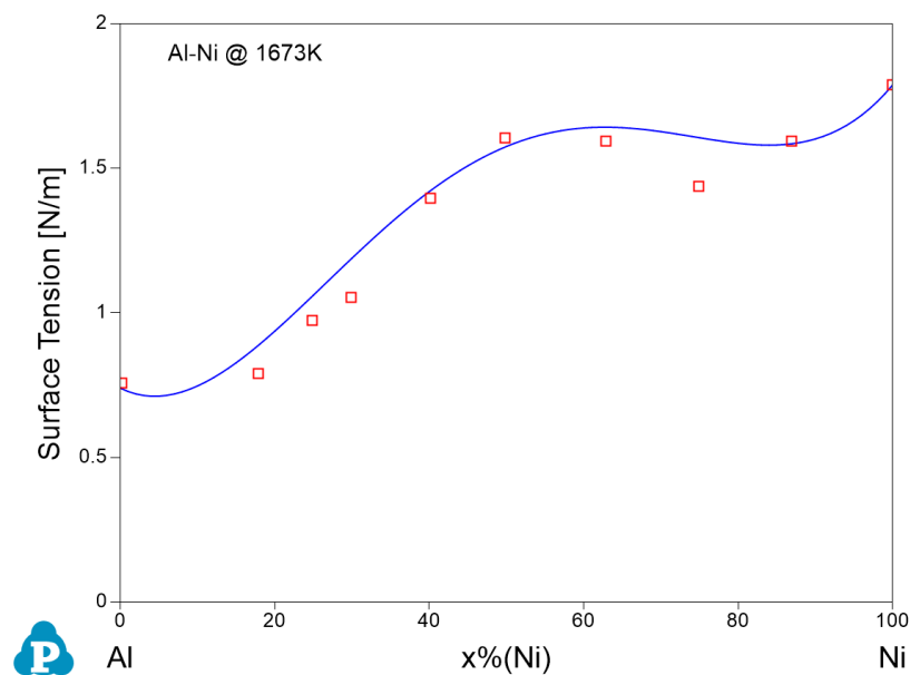
Figure 3.3: Surface tension of Al-Ni alloys
