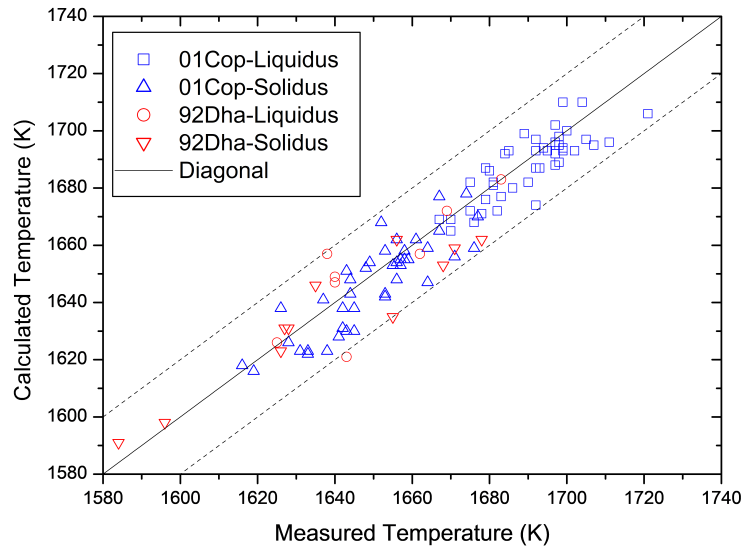
Figure 1.1: Comparison between the calculated and experimentally measured liquidus and solidus temperatures
