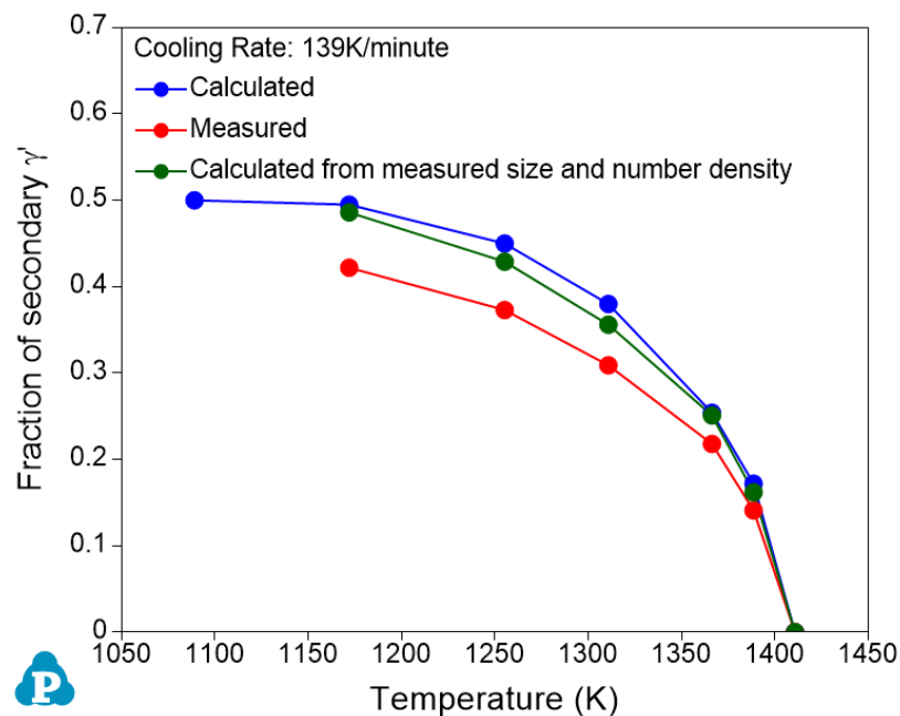
Figure 2.3: Comparison between the simulated and the measured volume fractions of \gamma' with the cooling speed of 139K/m to different temperatures
