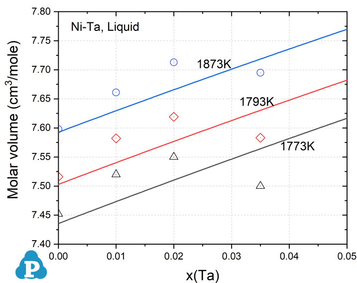
Figure 3.1: Molar volume of Ni-Ta liquid alloys [2004Muk, 2005Fan]
