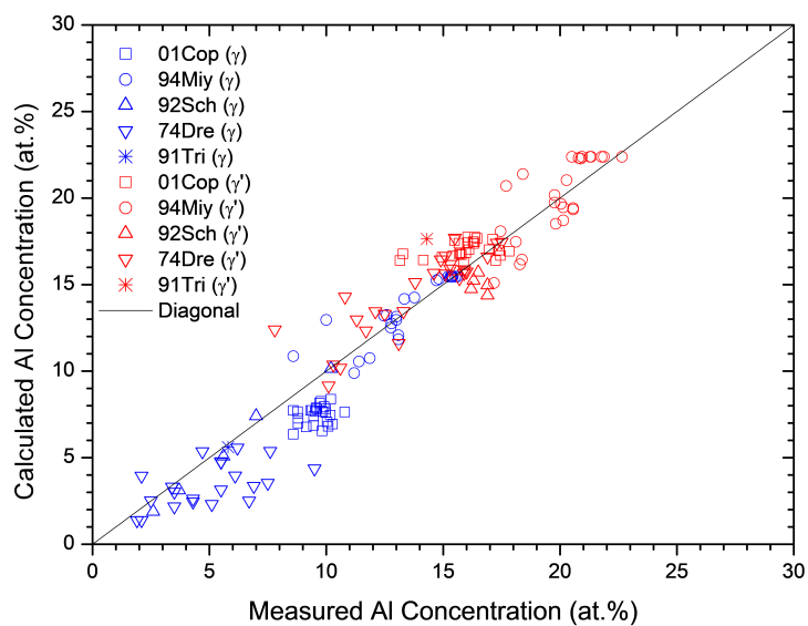
Figure 1.4: Comparison between the calculated and experimentally measured equilibrium compositions of Al in \gamma and \gamma' phase
