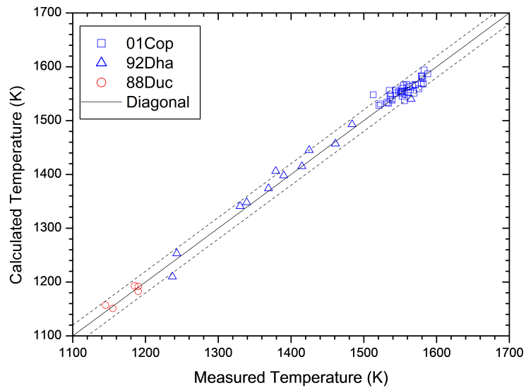
Figure 1.2: Comparison between the calculated and experimentally measured solvus temperatures of the \gamma' phase
