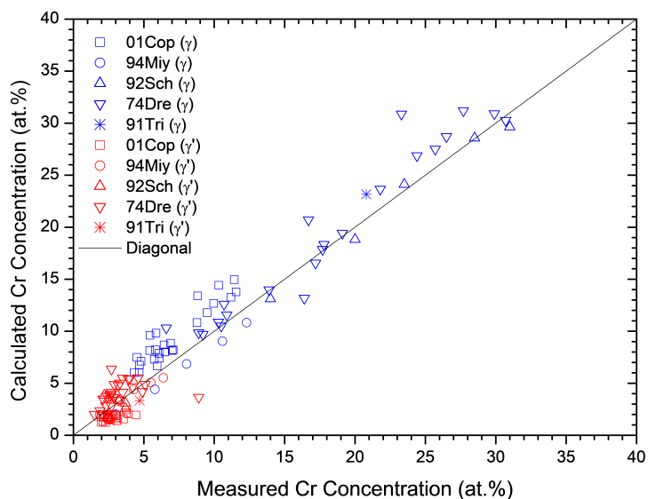
Figure 1.6: Comparison between the calculated and experimentally measured equilibrium compositions of Cr in \gamma and \gamma' phases
